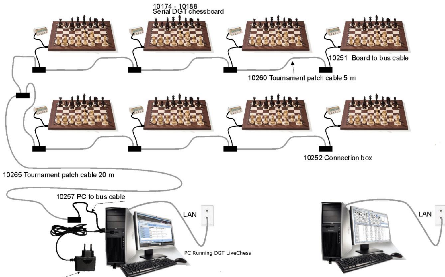
FIGURE 1 WIRING BETWEEN THE DGT E-BOARDS AND PCS
